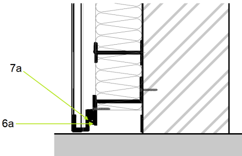
Figure 5. Bottom of Wall Assembly
