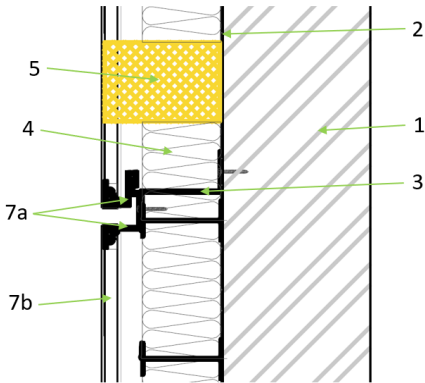
Figure 3. Wall Assembly
