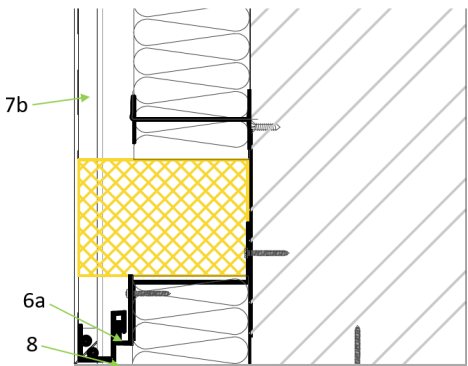
Figure 2. Top of Opening
