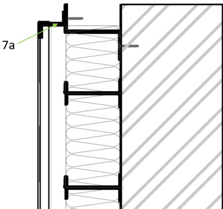
Figure 1. Top of Wall Assembly
