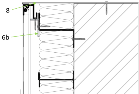
Figure 4. Bottom of Opening
