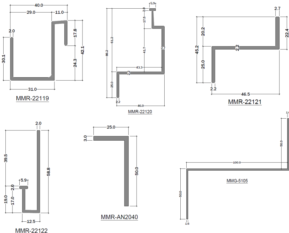
Figure 6. Extrusions (All dimensions are in mm)
